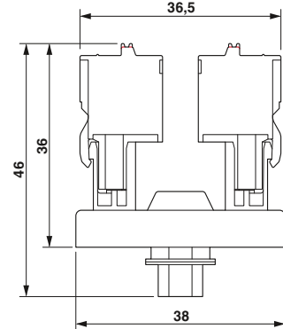
Dimensional drawing DFLK-D...SUB...FKCT
