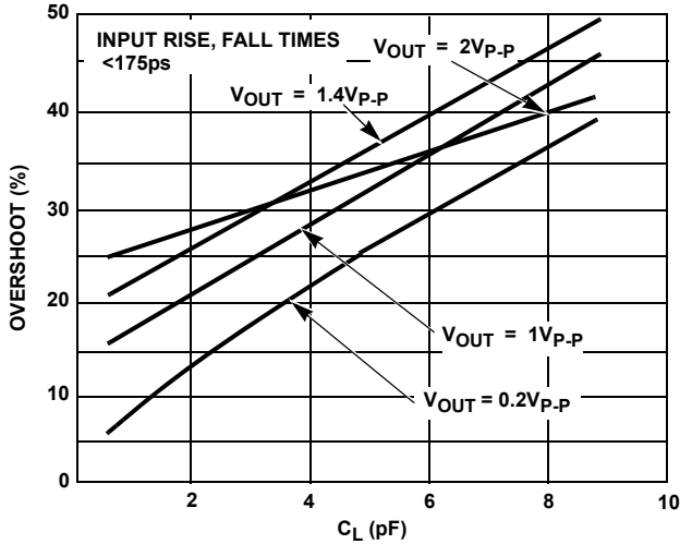
FIGURE 20. PULSE OVERSHOOT vs V_{OUT}, C_L; R_L = 500\Omega
