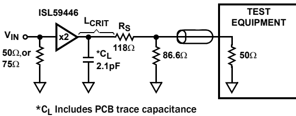
FIGURE 29D. 150Ω TEST CIRCUIT WITH 50Ω LOAD
