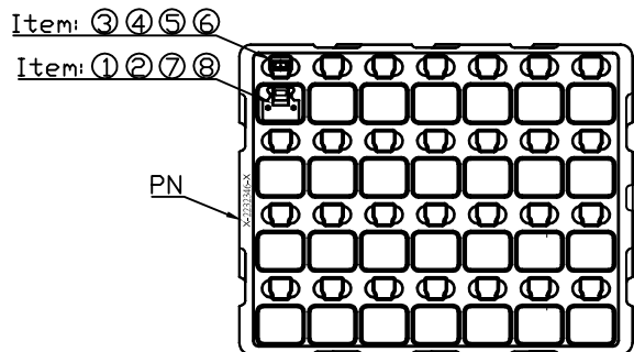
TRAY:400X315X25
